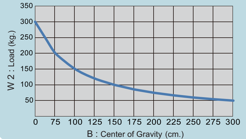
PPR-300 Center of Gravity
