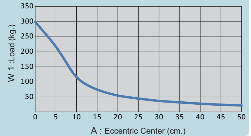
PPR-300 Positioner Eccentric Load
